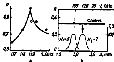
Fig. 8. Probability of hemolytic activity change by low-intensity MMR irradiation (for the threshold of likelihood ratio function L_0 = 1 ) and variation of optical density R of specimens with Proteus "irradiated" by human inductor through filters 5 and 7.
