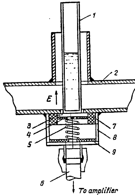
FIG. 1. Schematic representation of the recording node of the mechanical vibrations excited in a liquid: 1—tube containing liquid; 2—rectangular waveguide; 3—piezo crystal; 4—rubber ring; 5—spring; 6—h.f. cable; 7—centring ring; 8—screen; 9—insulating washer.
