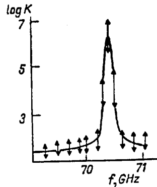
FIG. 1. Induction coefficient of lambda prophage as a function of the frequency of the acting radiation [11].
