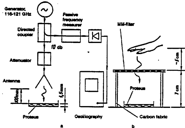
Fig. 7. Setup for irradiation of bacteria (a) and experiments to detect BII (b).
